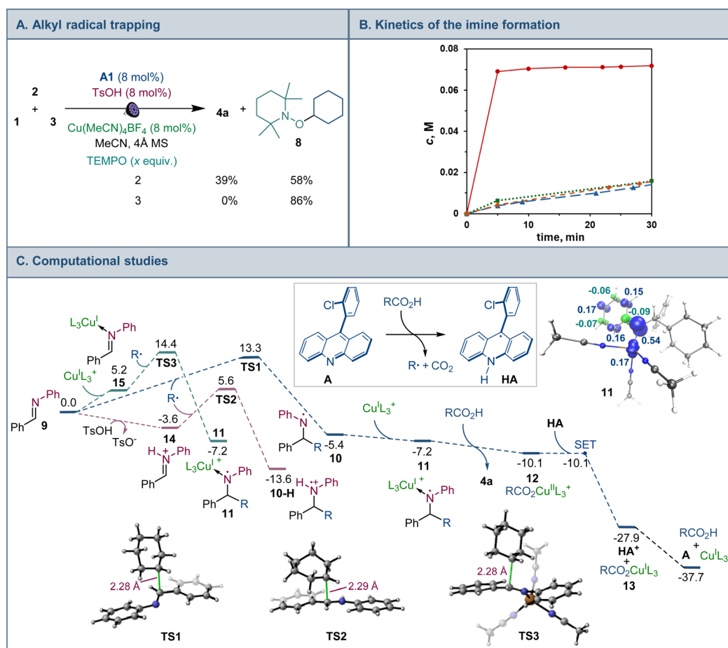
Fig. 3 (A) Mechanistic studies of the tri-component amine construction. (B) Kinetic profile of imine 9 formation. — with TsOH (8 mol%); — with acid 3 (1 equiv.); — with Cu(MeCN) 4 BF 4 (8 mol%); — uncatalyzed reaction. (C) Computational studies of the radical amine formation, \Delta G , kcal mol -1 , and the spin density isosurface (isoval = 0.05) for intermediate 11 . R = cyclohexyl, L = MeCN.
