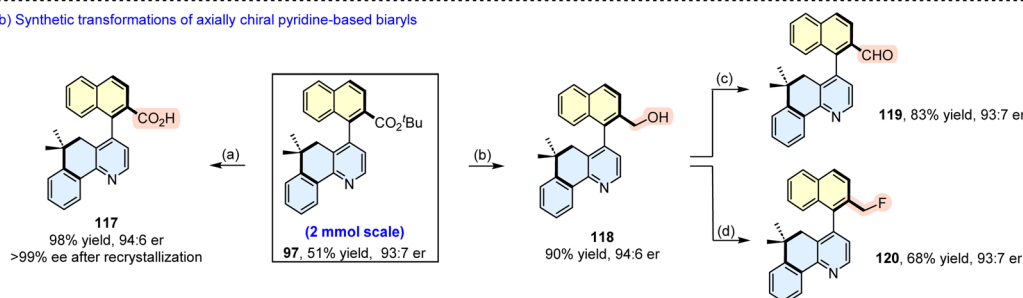
Scheme 9 (a) Construction of axially chiral pyridine-based biaryls. Reaction conditions: oxime ester (0.6 mmol), enal (0.2 mmol), \text{Fe}(\text{acac})_3 (10 mol%), A4 (20 mol%), 1,4-dioxane/toluene (2 mL, v/v = 1/1 ), 50 °C, 48 h, under \text{N}_2 . (b) Synthetic transformations of 97 . Reaction conditions: (a) NaOH (2 M), 95% EtOH, 100 °C, 24 h. (b) DIBAL-H (2.5 equiv.), DCM, -78 °C, 2 h. (c) IBX (1.2 equiv.), HOAc (1.2 equiv.), MeCN, rt, 6 h. (d) DAST (4 equiv.), DCM, 0 °C to rt, 12 h.
