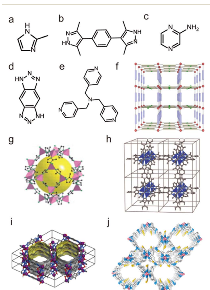
Fig. 9 The structures of representative Co(II)-MOFs and the used ligands. (a) The MeIM ligand. (b) The H 2 bdpb ligand. (c) The pyz-NH 2 ligand. (d) The H 2 bpta ligand. (e) The TPMA ligand. (f) ZJU-75. Reproduced from ref. 124 with permission from Wiley, Copyright 2023. (g) ZIF-67. Reproduced from ref. 120 with permission from The American Association for the Advancement of Science, Copyright 2008. (h) MFU-1. Reproduced from ref. 121 with permission from Wiley, Copyright 2009. (i) MAF-X27-Cl. Reproduced from ref. 122 with permission from the American Chemical Society, Copyright 2016. (j) FJIH-30. Reproduced from ref. 123 with permission from the American Chemical Society, Copyright 2020.
