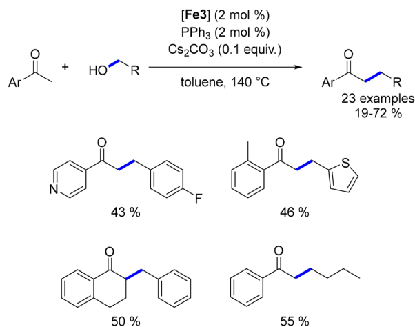
Scheme 80 Alkylation of ketones, as reported by Renaud.
