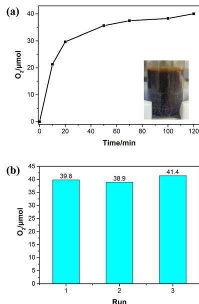
Fig. 3 (a) The time-dependent photocatalytic O_2 evolution and (b) recycling performance of CoBIM-1 .
