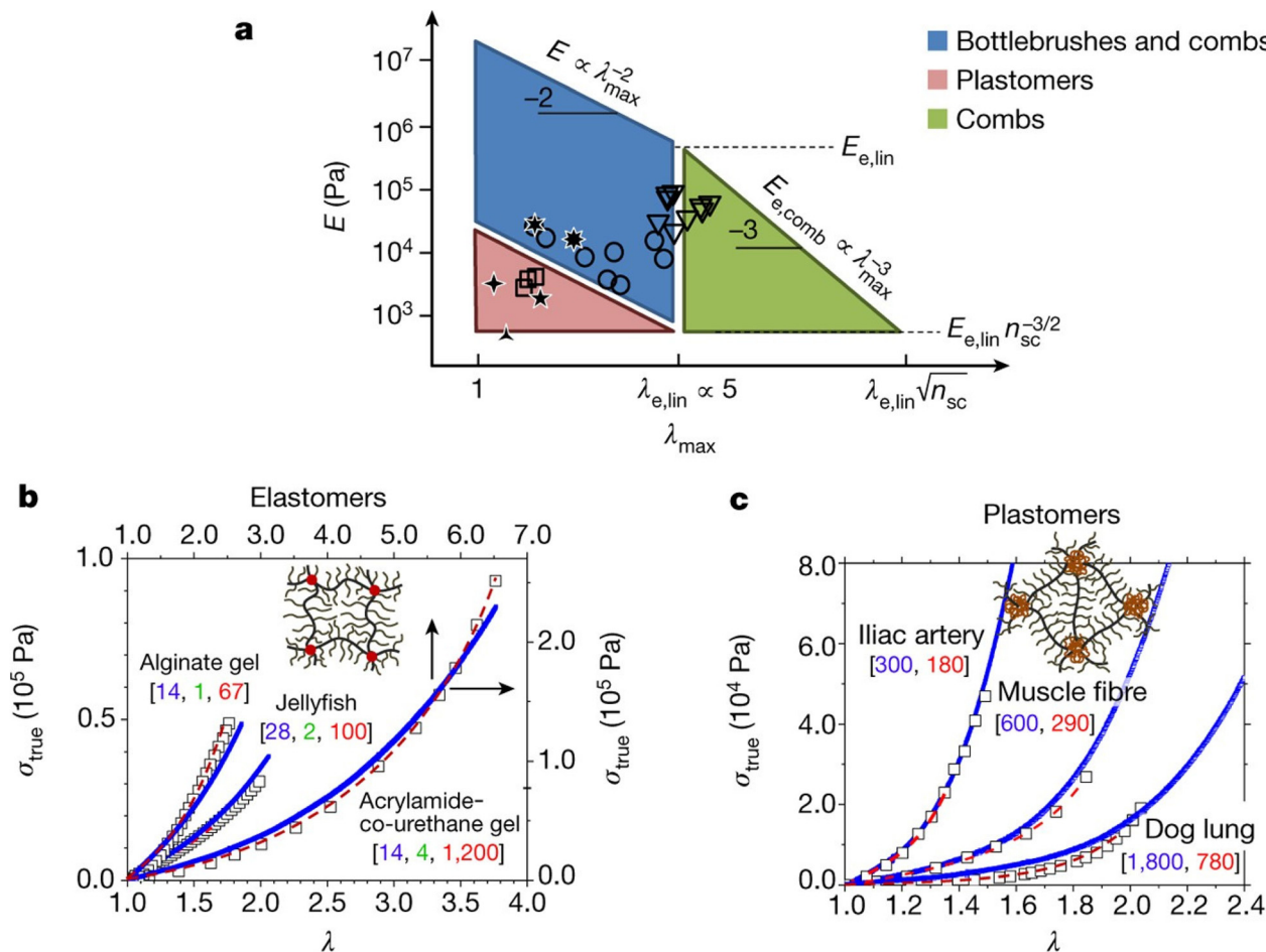
Fig. 4 (a) PDMS bottlebrushes, combs and elastomers with the mechanical properties of biological materials. This graph shows these properties (circles, bottlebrushes with n_g < 2 ; triangles, combs with n_g > 2 ; squares, ABA copolymers (plastomers)), along with the properties of brain, arteries, lungs, eye lens and jellyfish. The \lambda_{\max} boundaries correspond to the elongations-at-break of conventional linear-chain networks ( \lambda_{e,\text{lin}} \approx 5 ) and comb-like networks that result from entanglements of the network strands. The E boundaries correspond to the entanglement plateau moduli of linear chain ( E_{e,\text{lin}} ) and comb-like chain melts. The diagonal boundaries are provided by inverse E and \lambda_{\max} relationships of linear and comb-like networks. The lower boundary of the blue parallelogram, Pa, corresponds to bottlebrush networks with long side chains of about 100 units. (b) Stress-strain data (squares) for alginate gel, jellyfish tissue and poly(acrylamide-co-urethane) gel, together with fitting analysis of the data (dashed red lines), and curves for PDMS bottlebrush and combs synthesized via fitting analysis with the indicated architectural [nsc, ng, nx] triplets (blue lines). (c) Stress-strain data (squares) for iliac artery, muscle and dog lung tissue, together with fitting results obtained (dashed red lines), and stress-strain curves from PMMA-PDMS-PMMA mimics (solid blue lines) with different degrees-of-polymerization of the PDMS bottlebrush backbone (nbb) and PMMA linear chains (N) as indicated by [nbb, N]. Each experimental curve in (b) and (c) represents the average of at least three measurements with a relative standard deviation of less than 5% (reproduced from ref. 88 with permission from Springer Nature, copyright 2017).
