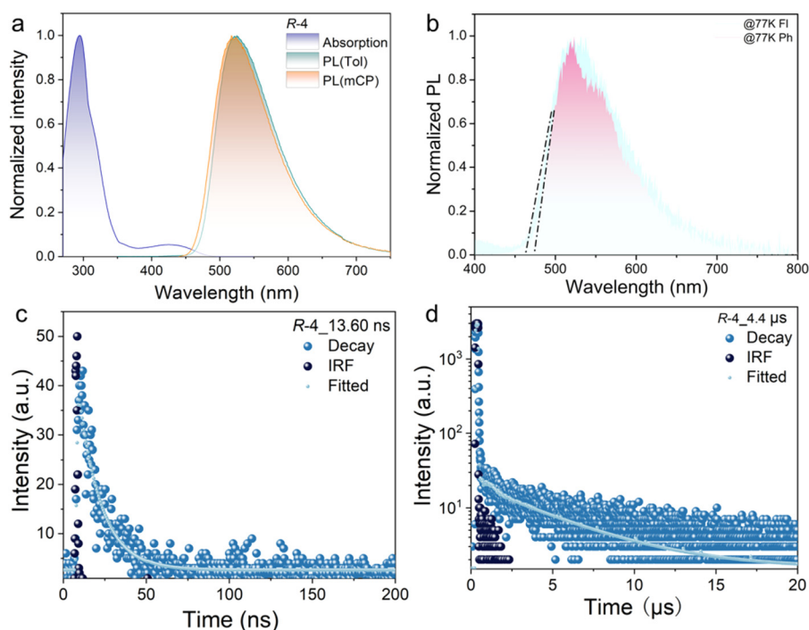
Fig. 4 (a) UV-vis spectra and PL spectra of R-4 measured in toluene solution ( 10^{-5} M) and 5 wt% doped in mCP film ( \lambda_{ex} = 420 nm); (b) low-temperature fluorescence (Fl) and phosphorescence (Ph) of R-4 doped in mCP film ( \lambda_{ex} = 370 nm, delayed 2 ms); and (c) and (d) transient PL decay curves ( \lambda_{ex} = 420 nm) of 5 wt% R-4 doped in mCP film.
