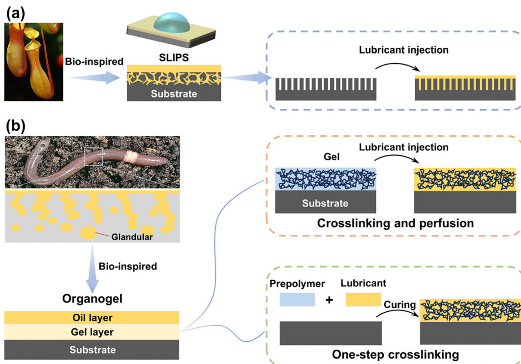
Fig. 14 Schematic representation of the bio-inspired surfaces: (a) SLIPSS and (b) organogels and their preparation methods.
