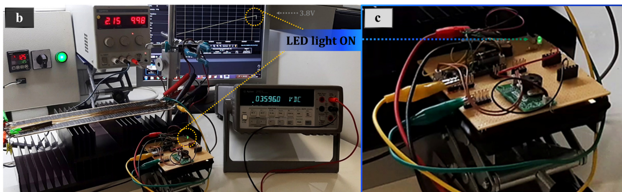
Fig. 8 (a) Diagram of the time required to charge the ALD-EH4295 utilizing the energy generated by the GFRP-GTEG to power up an LED at various \Delta T s. (b) and (c) The electronic board and the experimental setup containing the ALD-EH4295 employed at \Delta T = 100 °C to light up a green LED.
