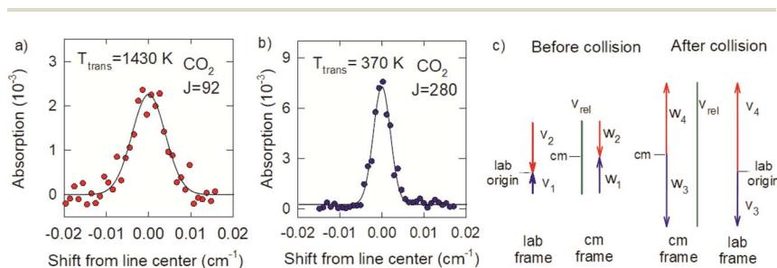
Fig. 11 Doppler-broadened line profiles for CO 2 (a) J = 92 and (b) J = 280 at 200 ns following the optical centrifuge pulse. (c) Velocity vectors in the lab frame ( v ) and center of mass (cm) frame ( w ) for a collision with b = 0 of an optically centrifuged molecule and a thermal bath molecule, before (1, 2) and after (3, 4) collisional energy transfer.
