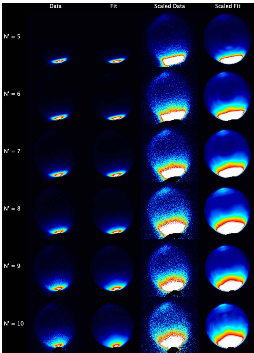
Fig. 2 Experimental data and fits. (Left to right) Summed V + H data; summed V + H fit; scaled summed V + H data; scaled summed V + H fit. (Top to bottom) Final states N' = 5 to 10 . The individual experimental measurements for each N' have been fitted independently as described in the text, and the relevant images summed for presentation here. For example, the N' = 10 images are the result of fitting to 10 V and H polarization pairs of images, and the data and fit images presented are therefore each the sum of 20 images. The rescaled images have their maximum intensity set to 1/15 th ( N' = 5 and 6 ), 1/10 th ( N' = 7 and 8 ) and 1/5 th ( N' = 9 and 10 ) of the data image maximum, respectively. NO beamspot subtraction artefacts have been masked.
