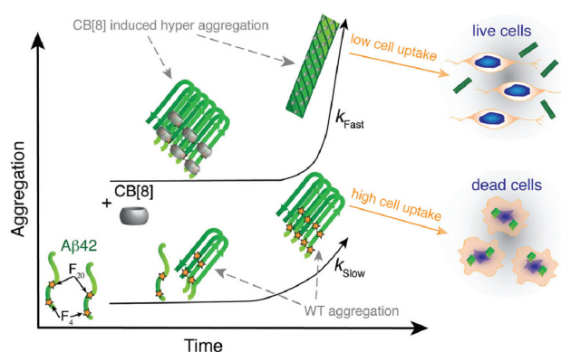
Fig. 29 Time-based aggregation of Aβ 1-42 in the presence and absence of Q8. Q8 induces the aggregates to grow faster and larger, and cell uptake and toxicity are reduced. CB[8] is Q8. 136 Reproduced from ref. 136 with permission from the Royal Society of Chemistry.
