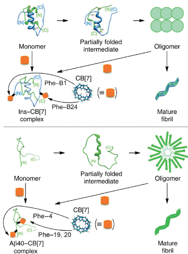
Fig. 28 Schematic for the inhibition of fibrillation using Q7 to stabilize the monomeric forms of (top) insulin and (bottom) Aβ 1-40 . CB[7] is Q7. 132 Reproduced with permission from ref. 132. © 2014 Wiley-VCH Verlag GmbH & Co. KGaA, Weinheim.
