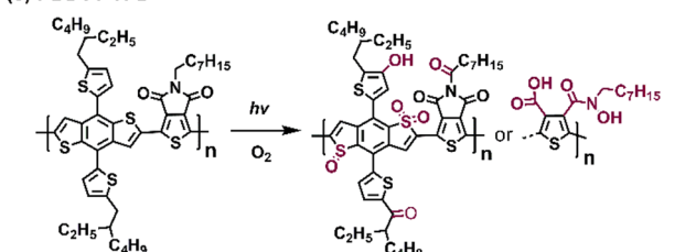
Fig. 19 Photodegradation products (with O_2 ) of five different D–A type polymer donors. 146
