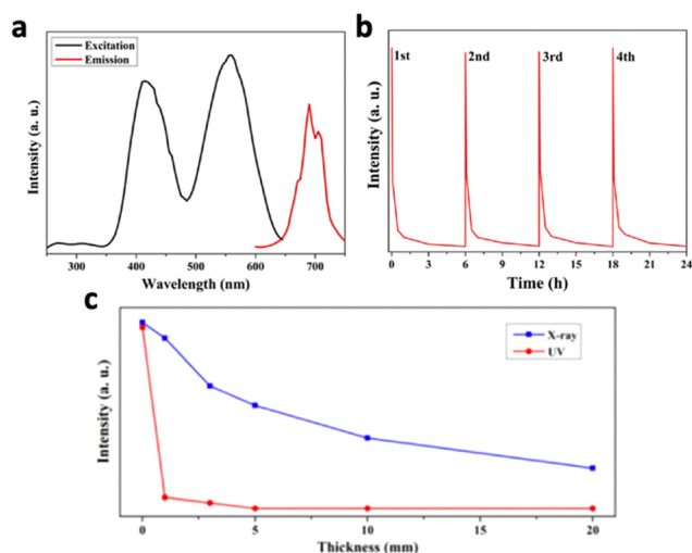
Fig. 18 (a) Excitation spectrum (black) and emission spectrum (red) of \text{ZnGa}_2\text{O}_4:\text{Cr}^{3+} . (b) 4 Cycles of persistent luminescence decay curves by \text{ZnGa}_2\text{O}_4:\text{Cr}^{3+} following cessation of X-ray irradiation (5 min, 45 kVp). (c) Luminescence intensity of \text{ZnGa}_2\text{O}_4:\text{Cr}^{3+} excited by X-ray (blue) and 365 nm UV (red) through pork tissues with different thicknesses (0, 1, 3, 5, 10, and 20 mm). Reproduced with permission from ref. 211. Copyright 2017, American Chemical Society.
