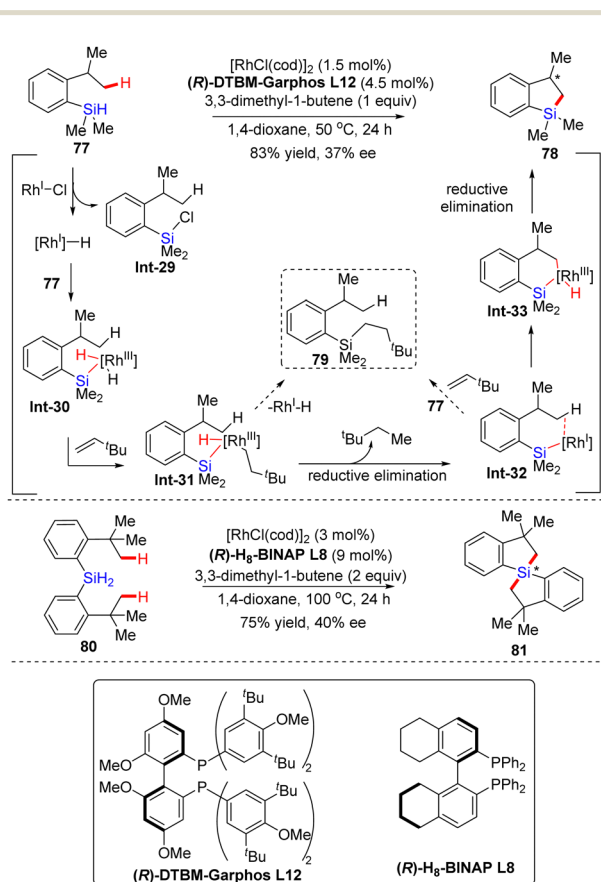
Scheme 24 Rh(i)-Catalyzed intramolecular C-H silylation of 2-isopropylphenylsilane and dihydrosilane.
