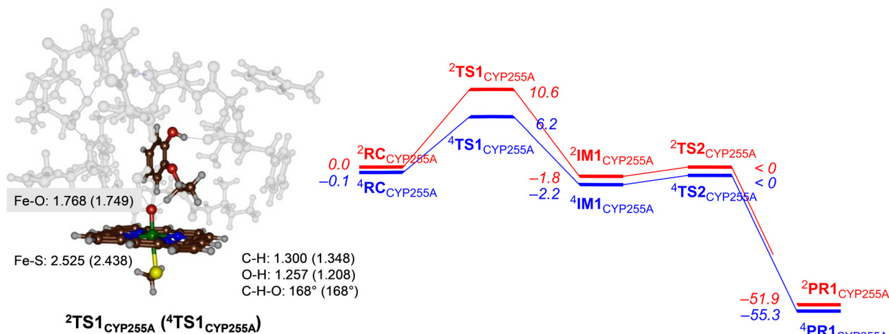
Fig. 3 UB3LYP calculated pathways for ethoxy group hydroxylation of guaethol by CYP255A wildtype model. Free energies (ΔG in kcal mol −1 ) are with energies at BS2 level of theory and with ZPE, thermal and entropic corrections included at 298 K. Also shown are optimized geometries of the rate-determining transition states with distances in Å and angles in degrees.
