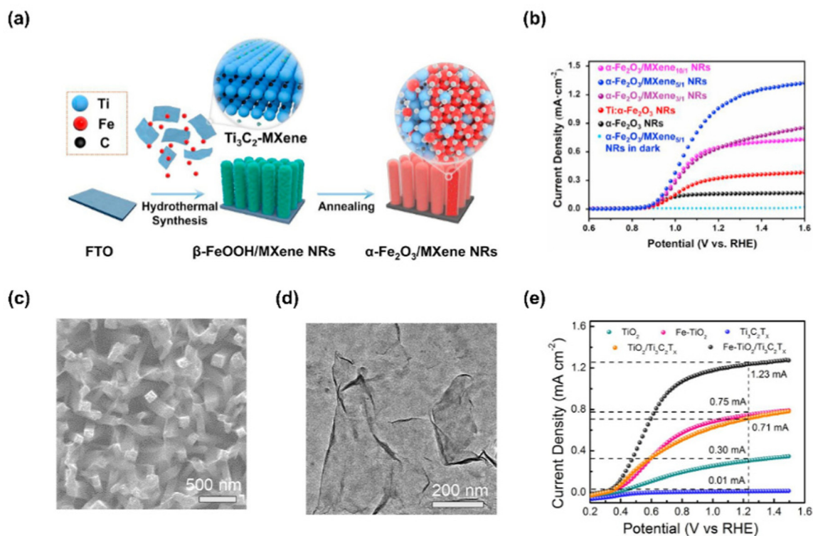
Fig. 11 (a) Schematic of fabrication process for \alpha\text{-Fe}_2\text{O}_3/\text{MXene} , NRs. (b) LSV curves \alpha\text{-Fe}_2\text{O}_3 , NRs, \text{Ti}_3\text{-}\alpha\text{-Fe}_2\text{O}_3 , \alpha\text{-Fe}_2\text{O}_3/\text{MXene}_{5/1} NRs, \alpha\text{-Fe}_2\text{O}_3/\text{MXene}_{10/1} NRs, and \alpha\text{-Fe}_2\text{O}_3/\text{MXene}_{10/1} NRs. Copyright 2021, Elsevier. (c) SEM image of the Fe- \text{TiO}_2/\text{Ti}_3\text{C}_2\text{T}_x . (d) TEM image of the exfoliated \text{Ti}_3\text{C}_2\text{T}_x nanosheets. (e) LSV curves of \text{TiO}_2 , \text{Ti}_3\text{C}_2\text{T}_x , \text{TiO}_2/\text{Ti}_3\text{C}_2\text{T}_x , Fe- \text{TiO}_2 (Fe: 5 mol%) and Fe- \text{TiO}_2/\text{Ti}_3\text{C}_2\text{T}_x . Copyright 2022, Elsevier.
