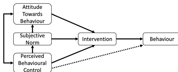
Fig. 3 Ajzen's Theory of Planned Behaviour (Ajzen 1991).
