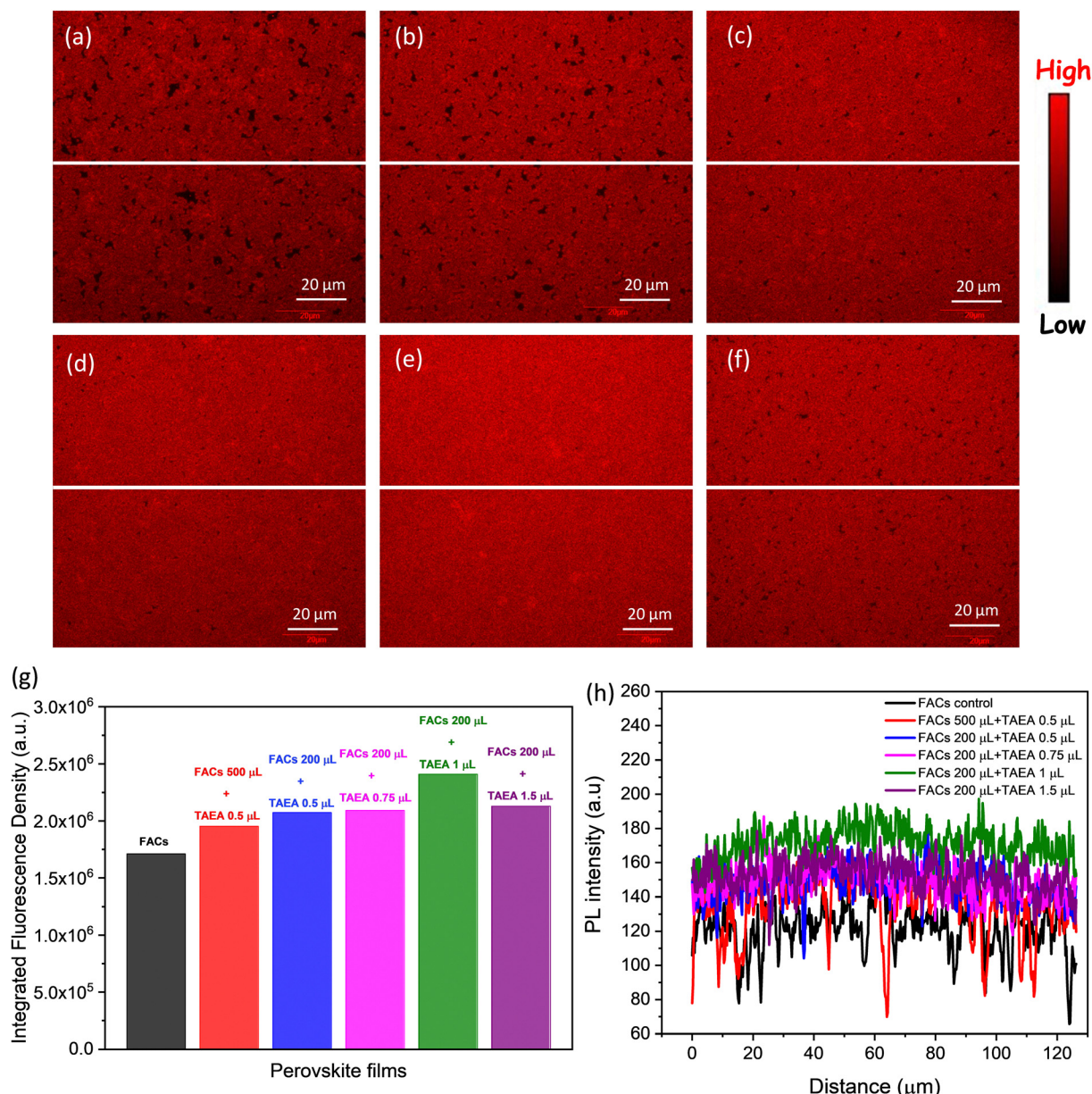
Fig. 5 SCLM PL intensity maps of (a) FACS film, FACS film containing (b) 0.5 μL of TAEA in 500 μL of FACS precursor, (c) 0.5 μL of TAEA in 200 μL of FACS precursor, (d) 0.75 μL of TAEA in 200 μL of FACS precursor, (e) 1 μL of TAEA in 200 μL of FACS precursor, and (f) 1.5 μL of TAEA in 200 μL of FACS precursor. (g) Integrated fluorescence density in the films calculated in the 128 μm × 128 μm area of the sample. (h) PL line profile plotted along the breadth of the samples as denoted by the white horizontal lines in (a)–(f).
