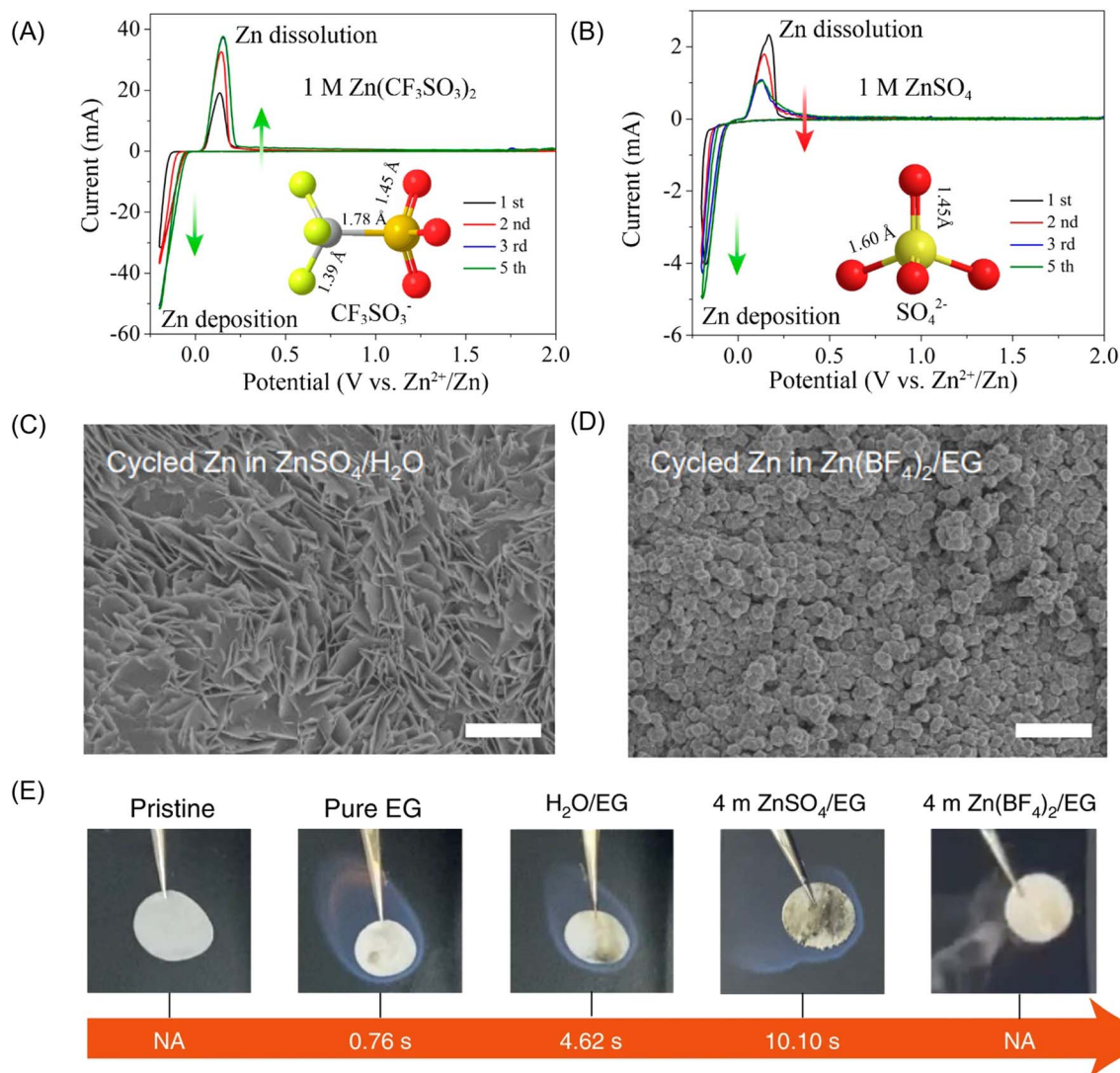
Fig. 6 Cyclic voltammery of the Zn electrode in aqueous electrolyte of (A) 1 M \text{Zn}(\text{CF}_3\text{SO}_3)_2 and (B) 1 M \text{ZnSO}_4 at the scan rate of 0.5 \text{ mV s}^{-1} between -0.2 and 2.0 \text{ V} . Reproduced with permission. 102 Copyright 2016, American Chemical Society. Top-view SEM images of the cycled Zn after 20 cycles in (C) the reference aqueous \text{ZnSO}_4 electrolyte and (D) the 4 m \text{Zn}(\text{BF}_4)_2/\text{EG} electrolyte. (E) Ignition tests of a pristine glass fibre separator, one saturated with pure EG, a \text{H}_2\text{O}/\text{EG} solution, a 4 m \text{ZnSO}_4/\text{EG} solution and a 4 m \text{Zn}(\text{BF}_4)_2/\text{EG} solution. NA (not applicable) indicates non-flammability. Reproduced with permission. 101 Copyright 2021, Springer Nature.
