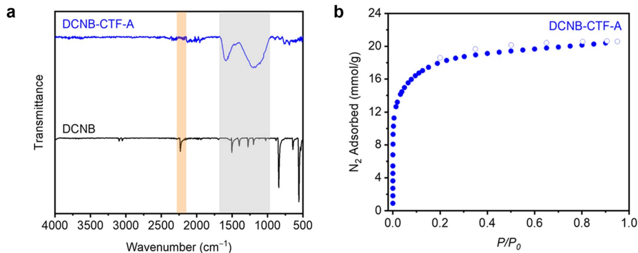
Fig. 6 Solid-state characterization of DCNB-CTF-A made with 5.00 equiv. of \text{ZnBr}_2 at 400 \text{ }^\circ\text{C} for 40 h. (a) ATR-IR spectra of DCNB and DCNB-CTF-A. The orange highlighted region shows the disappearance of the \text{C}\equiv\text{N} stretch from DCNB, and the gray highlighted region indicates the appearance of triazine stretches in DCNB-CTF-A. (b) 77 K \text{N}_2 adsorption (filled circles) and desorption (open circles) isotherms of DCNB-CTF-A.
