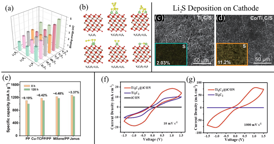
Fig. 13 (a) Three-dimensional columnar contrasts of the binding energy of several transition metal carbides for \text{LiPSs} . (b) Theoretical structure of \text{V}_4\text{C}_3\text{O}_2 and optimized configurations of \text{Li}_2\text{S}_n ( n = 1, 2, 4, 6, 8 ) adsorption on \text{V}_4\text{C}_3\text{O}_2 315 (Reproduced with permission from ref. 315. Copyright 2022, Elsevier). SEM images and the corresponding sulfur distribution map of the (c) \text{Ti}_2\text{C} and (d) \text{Co}/\text{Ti}_2\text{C} cathodes after \text{Li}_2\text{S} deposition 29 (Reproduced with permission from ref. 29. Copyright 2022, John Wiley and Sons). (e) Self-discharge tests of the LSBs with standard PP, Cu-TCPP-modified, MXene-modified, and Janus (Cu-TPP/MXene) separator configurations after resting for 120 h 317 (Reproduced with permission from ref. 317. Copyright 2023, Elsevier). CV curves of symmetric cells at a scan rate of (f) 10 \text{ mV s}^{-1} and (g) 1000 \text{ mV s}^{-1} for the \text{Ti}_3\text{C}_2@i\text{CON} and \text{Ti}_3\text{C}_2 -modified PP separators 318 (Reproduced with permission from ref. 318. Copyright 2021, John Wiley and Sons).
