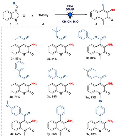
Scheme 3 Scope of the 3-ylidene oxindoles. Reaction conditions: unless otherwise specified, 3-ylideneoxindoles ( 1 ) (0.2 mmol), 2 (0.4 mmol), \text{DMAP} (0.24 mmol) and \text{PC4} (2 mol%) in 40 \mu\text{L} of water and 1.6 mL acetonitrile irradiated with a blue LED (455 nm) for 24 h under an argon atmosphere.
