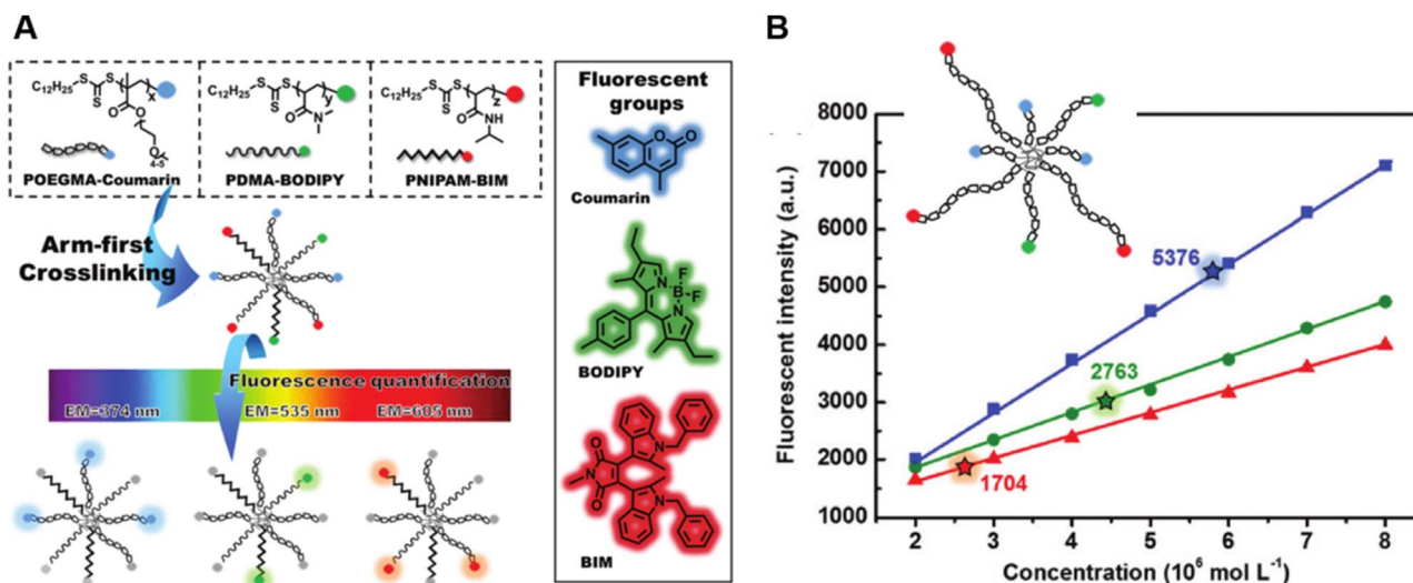
Fig. 6 (A) Illustration of the arm-first approach for the synthesis of miktoarm star polymers bearing different fluorescent end-groups. (B) Linear fits of fluorescence intensities of mikto-arm stars with the same monomeric units but different molecular weights, as shown in the inset, to quantify miktoarm star composition. Reproduced from ref. 184 with permission from The Royal Society of Chemistry, copyright 2022.
