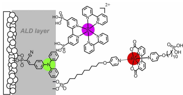
Fig. 23 Photoanodes employing a triphenylamine photosensitizer (green ball) bound to the semiconductor, a protective ALD layer used to anchor a Ru(bda) WOC (red ball) and a Ru(II) tris(bipyridine) redox mediator (purple ball). Reprinted from ref. 128 with permission from the Proceedings of the National Academy of Sciences (PNAS), copyright 2018.
