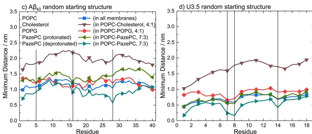
Fig. 6 (I) Average distances between the phosphate head groups of POPC in the outer membrane leaflet and the peptide C _{\alpha} atoms of (a) A \beta 40 and (b) U3.5 with random starting structures (perpendicular to the membrane along z-axis) during the last 10 ns simulation time of all replicates. (II) Average minimum distances between the peptides (c) A \beta 40 and (d) U3.5 with random starting structures and the lipid bilayer components POPC, cholesterol, POPG, and PazePC during the last 10 ns simulation time of all replicates. The vertical lines at residues 5 (arginine), 16 (lysine) and 28 (lysine) for A \beta 40 and at residues 7 (arginine), 8 (arginine) and 14 (lysine) for U3.5 indicate the positively charged residues in both peptides to guide identifying the closest peptide-membrane interactions. Note that the symbols are used to distinguish the data sets and each residue has a data point.
