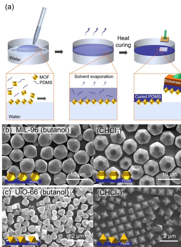
Fig. 16 (a) Scheme of preparation of oriented MOF–PDMS films. (b) SEM images of oriented MIL-96–PDMS films and (c) UiO-66–PDMS films prepared using butanol (left) and \text{CHCl}_3 (right) as a casting solvent. Adapted with permission from ref. 101. Copyright 2021, American Chemical Society.
