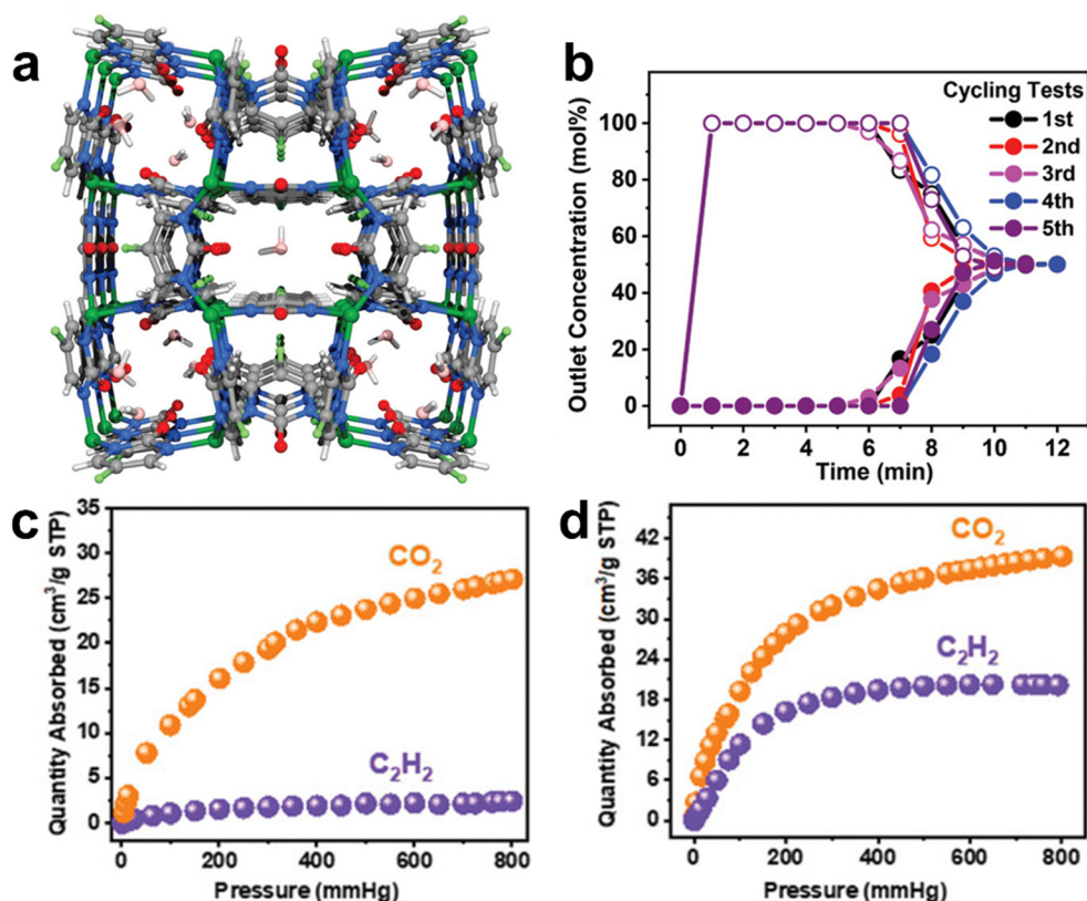
Fig. 11 (a) Schematic structure of Cu-F-pymo MOF with residual water molecules. (b) Breakthrough cycling tests of the equimolar \text{CO}_2/\text{C}_2\text{H}_2 mixture. (c) and (d) Separation performance toward \text{CO}_2 and \text{C}_2\text{H}_2 in Cu-F-pymo under different activation conditions. Reprinted with permission from ref. 143 Copyright 2021 Wiley-VCH.
