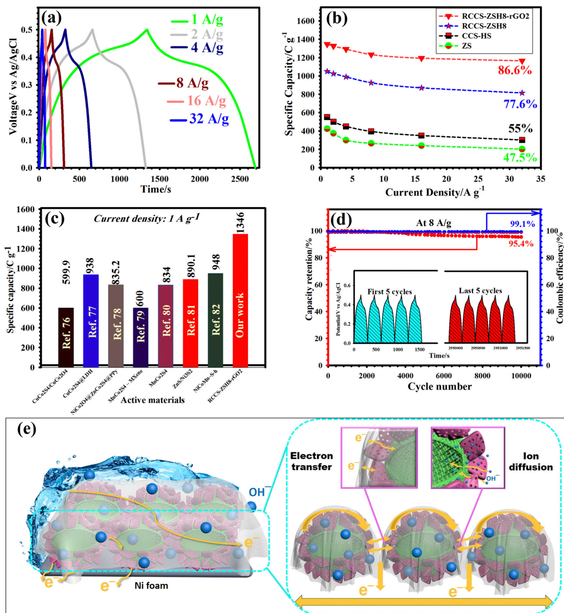
Fig. 7 (a) GCD profiles of the RCCS-ZSH8-rGO2 electrode from 1 to 32 \text{ A g}^{-1} . (b) Specific capacities vs. current densities of the ZS, CCS-HS, RCCS-ZSH8, and RCCS-ZSH8-rGO2 electrodes. (c) Comparison of capacity values of RCCS-ZSH8-rGO2 with the previous literature. (d) Longevity and Coulombic efficiency of the RCCS-ZSH8-rGO2 at 8 \text{ A g}^{-1} (the inset depicts the first and last 5 GCD cycles). (e) Schematic representation of the working mechanism of RCCS-ZSH8-rGO2 base-electrode.
