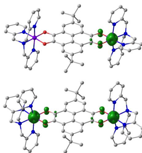
Fig. 9 Spatial structure and spin density distribution (contour value = 0.03 \text{e Å}^{-3} ) of compound 3 in the \{\text{Co}^{\text{III-LS}}(\text{tpa})\text{-pyrene}^{\text{Cat-Sq}}\text{-Co}^{\text{III-LS}}(\text{tpa})\} (top) and \{\text{Co}^{\text{II-HS}}(\text{tpa})\text{-pyrene}^{\text{Sq-Sq}}\text{-Co}^{\text{II-HS}}(\text{tpa})\} (bottom) charge distributions, as calculated by the DFT UTPSSH/6-311++G(d,p) method. Hydrogen atoms and counter-ions are omitted for clarity.
