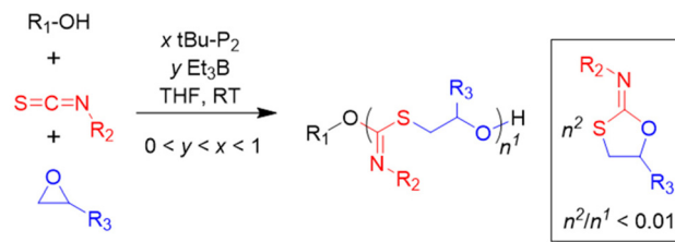
Scheme 15 Alternating copolymerization of epoxides and isothiocyanates to yield polythioimidocarbonates.
