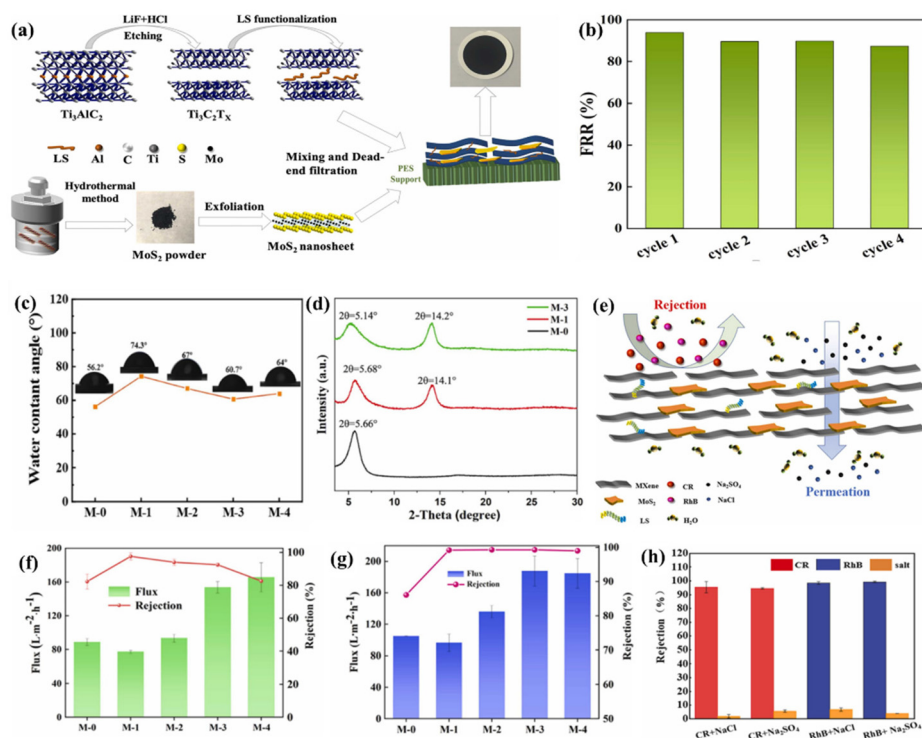
Fig. 11 (a) Scheme for the preparation of \text{MoS}_2\text{@LS-MXene} composite films by pressure-assisted self-assembly. (b) FRR data of M-3. (c) CA of all membranes. (d) XRD patterns of M-0, M-1, and M-3. (e) Separation mechanism of \text{MoS}_2\text{@LS-MXene} composite membranes. Removal rates of dyes by different membranes: (f) CR and (g) RhB, and (h) separation of dye/salt mixture with M-3. Reprinted with permission. 163 Copyright 2022, Elsevier.
