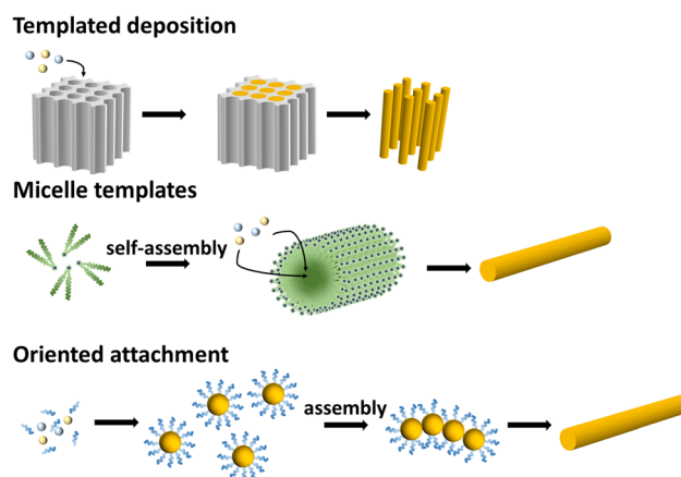
Fig. 3 Schematics illustrating the formation mechanisms that form the metal alloy nanowires directly with chemical methods.
