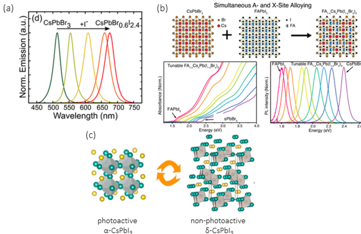
Fig. 13 (a) Variation of the PNC bandgap by alloying \text{Br}^- and \text{I}^- X-site, 253 and (b) by alloying concomitantly \text{Br}^- and \text{I}^- in the X-site and \text{FA}^+ and \text{Cs}^+ in the A-site. 254 (c) Spontaneous conversion of the photoactive to the non-photoactive phase of \text{CsPbI}_3 . 269 (a) Reproduced with permission from ref. 253. Copyright 2018 American Chemical Society. (b) Reproduced with permission from ref. 254. Copyright 2019 American Chemical Society. (c) Reproduced with permission from ref. 269. Copyright 2019 American Chemical Society.
