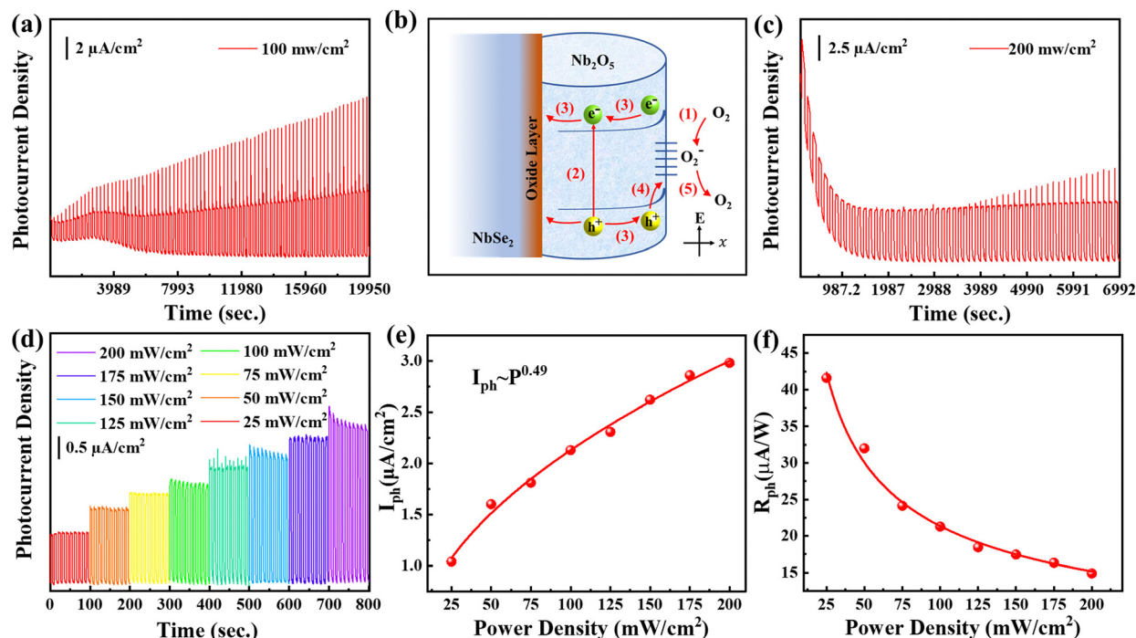
Fig. 7 (a) Long cycling stability measurement in a low oxygen environment, (b) OSCPC mechanism, (c) long cycling stability measurement in enough oxygen environment, (d) light intensity-dependent photocurrent density, and (e) I_{ph} and (f) R_{ph} values extracted from (d).
