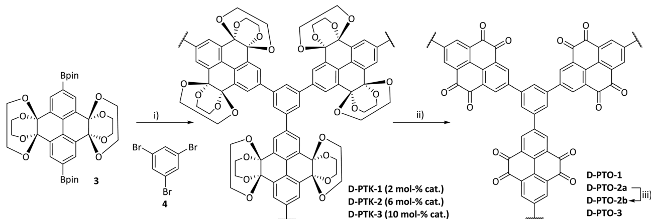
Scheme 2 Model compounds 1 and 2 and D-PTO synthesis (conditions: (i) 2–10 mol% Pd 2 (dba) 3 , 1 M K 2 CO 3 , THF, Ar, 85 °C, 14–18 h, 85%. (ii) 1. TFA/H 2 O (9:1), 24 h, rt, 2. 1 M H 2 SO 4 , 1 h, rt, 95%). (iii) Soxhlet extraction (MeOH, THF, Et 2 O). D-PTO-1 , -2a and -3 were prepared from the corresponding D-PTK-1 , -2 , and -3 batch, respectively.
