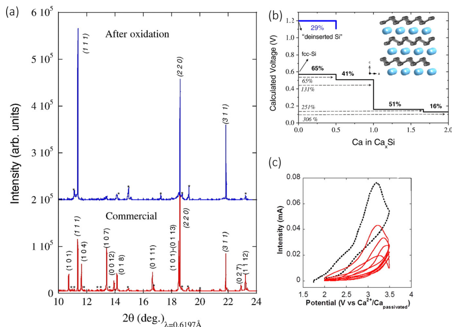
Fig. 9 (a) XRPD patterns; pristine anode prepared with the commercial \text{CaSi}_2 before (bottom) and after oxidation to 3.5 V vs. \text{Ca}^{2+}/\text{Ca} at 100 °C (top). Miller indices – \text{CaSi}_2 (roman type) and Si Peaks (marked as *) indicate impurities present in the pristine commercial sample. The pristine powder composed of \text{CaSi}_2 (70%) and Si (30%). (b) Calculated composition–voltage profiles. The black line corresponds to the calcination of fcc-Si following an alloying mechanism in which intermetallics \text{Ca}_x\text{Si} are formed. The blue line accounts for the deinsertion of Ca ions from the layered \text{CaSi}_2 . The inset shows the schematic crystal structure of \text{CaSi}_2 (Si in grey, Ca in blue). (c) Cyclic voltammograms ( 0.05 \text{ mV s}^{-1} ) of \text{CaSi}_2 electrode in a 2-electrode Ca cell operating at 100 °C. Reproduced with permission from ref. 89, copyright 2016 Elsevier B.V.
