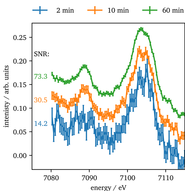
Fig. 8 Vtc spectra of Fe 2 O 3 at 75 GPa for different integration times. The SNRs are calculated for the maximum of the Kβ 2,5 emission with the background averaged between 7100 eV and 7110 eV. The data have been offset by 0.05 units for clarity.
