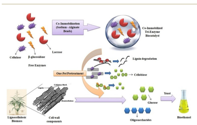
Fig. 23 Immobilization of co-immobilized laccase, cellulase, and \beta -glucosidase for ethanol production. Reproduced from ref. 255 with permission from Elsevier, copyright 2018.
