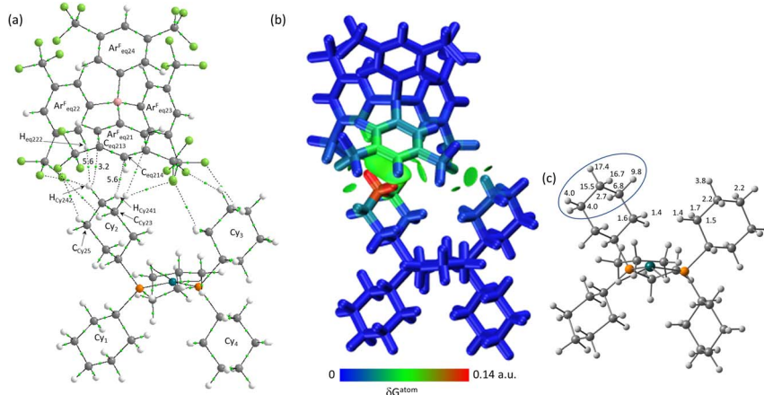
Fig. 8 (a) QTAIM molecular graph with Eq-2 in [1- propane ][ BAR F 4 ] - with BCPs in green and showing selected atoms and BCP electron densities (a.u. \times 10^{-3} ). Bond paths with \rho(r) < 0.001 a.u., intramolecular bond paths and ring critical points (RCP) are omitted for clarity. (b) IGMH plot where the cation and anion are defined as separate fragments. Sign( \lambda_2 ) \rho -coloured isosurfaces are plotted with \delta G^{\text{inter}} = 0.003 a.u. and atoms are coloured by \delta G^{\text{atom}} . (c) % \delta G^{\text{atom}} contributions on the cation that are above 1%, with the propylene motif highlighted (see text for details).
