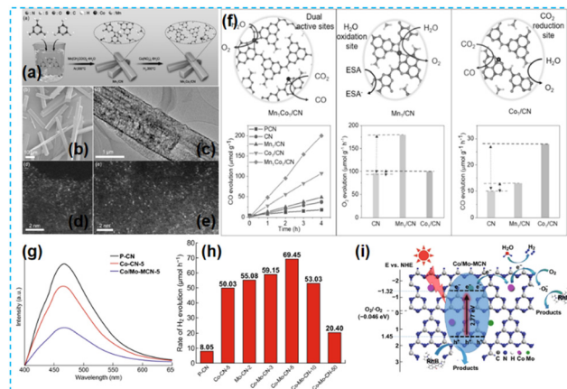
Fig. 27 (a) Synthesis of the Mn 1 Co 1 /CN catalyst. (b) SEM and (c) TEM images of Mn 1 Co 1 /CN. AC HAADF-STEM image of (d) Mn 1 /CN and (e) Mn 1 Co 1 /CN. (f) Photocatalytic activities of samples with double single-atom active sites for CO 2 reduction. 110 (g) Photoluminescence spectra of P-CN, Co-CN-5, and Co/Mo-MCN-5. (h) Photocatalytic H 2 evolution rate of the as-prepared materials. (i) Photocatalytic mechanism scheme of Co/Mo-MCN under visible light irradiation. 111
