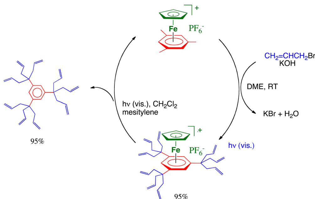
Scheme 5 \text{CpFe}^{\text{II}} -induced nona-allylation of mesitylene. The cationic charge of the \text{Fe}^{\text{II}} complex activates benzylic deprotonation by the base, followed by nucleophilic substitution of \text{Br}^- in \text{CH}_2=\text{CHCH}_2\text{Br} , this sequence proceeding 9 times in situ under ambient conditions. The resulting nona-allylated complex is then photolyzed by visible light in \text{CH}_2\text{Cl}_2 in the presence of mesitylene to produce the iron-free nona-allylated arene, which also regenerates the starting sandwich complex of mesitylene.
