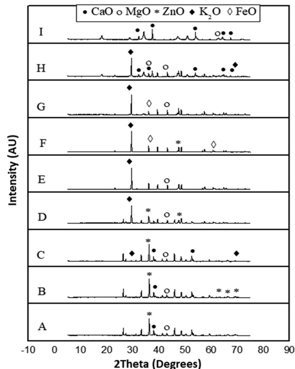
Fig. 3 XRD patterns of the calcined Archachatina marginata shells at (A) 100 °C, (B) 200 °C, (C) 300 °C, (D) 400 °C, (E) 500 °C, (F) 600 °C, (G) 700 °C, (H) 800 °C and (I) 900 °C.
