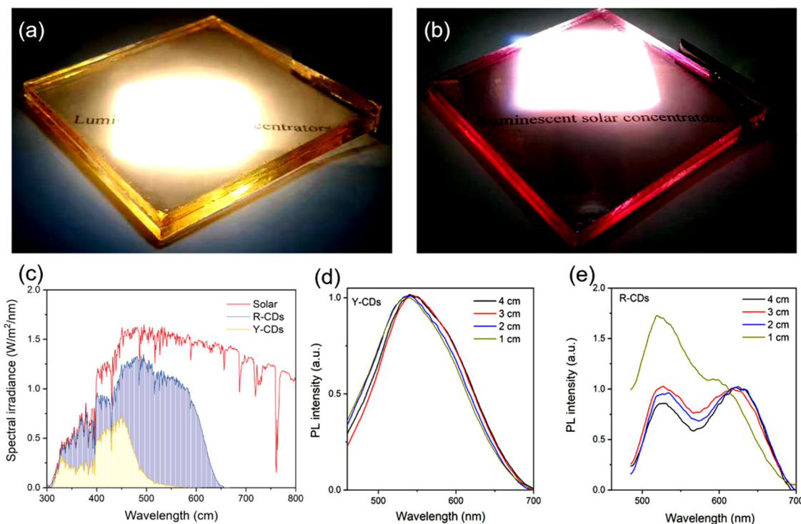
Fig. 12 Photographs of the laminated LSC based on yellow (a) and red C-dots (b) upon one sun illumination. Laminated LSC dimensions, 10 \times 10 \times 0.9 \text{ cm}^3 . (c) Calculated solar absorption of the LSCs and solar spectrum. The concentration of the C-dots in PVP was 1 wt% in PVP. PL spectra measured at different L for the yellow (d) and red C-dot (e) based LSCs. The excitation wavelength is 400 nm. Reproduced with permission from ref. 33. Copyright 2021, Royal Society of Chemistry.
