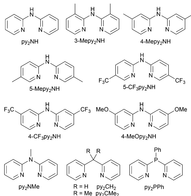
Scheme 16 Structures of di(pyridin-2-yl)amine N^{\wedge}N ligands.
