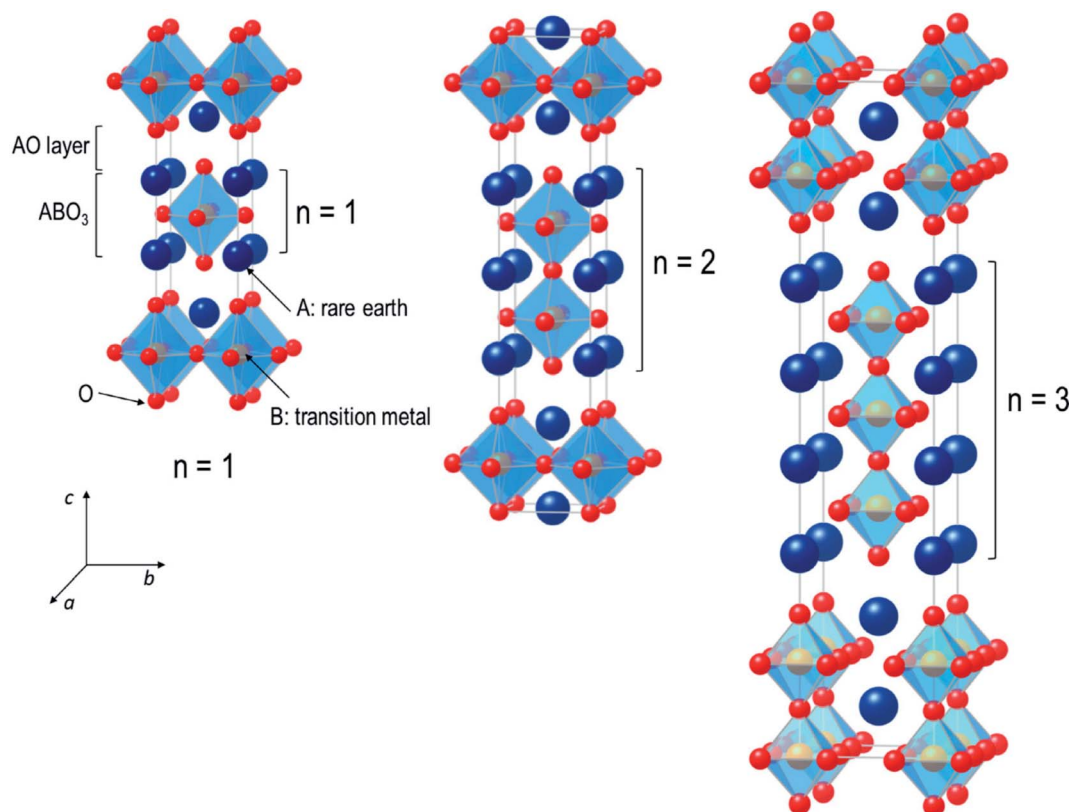
Fig. 6 Schematic crystal structures of n = 1, 2 and 3 members of layered structure Ruddlesden–Popper type \text{A}_{n+1}\text{B}_n\text{O}_{3n+1} perovskite oxides. The denotation of n represents the number of stacked perovskite \text{ABO}_3 layers separated by a rock salt AO layer. 250
