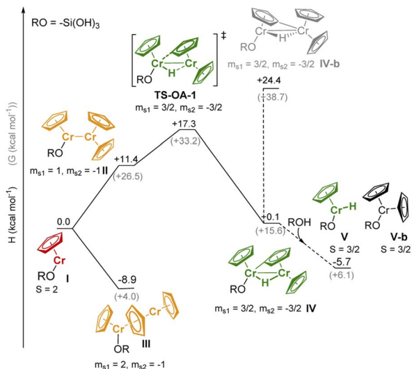
Fig. 4 Proposed reaction pathways for the interaction of 1 on partially dehydroxylated silica. Enthalpies ( H kcal \text{mol}^{-1} ) and free energies ( G kcal \text{mol}^{-1} ) are calculated with respect to I and \text{CrCp}_2 . For monomeric sites, the spin quantum number is indicated with S ; for dimeric sites, the local projection of the spin, as obtained from the Mulliken spin density on [\text{CrCp}] fragments I , is shown with m_{s_i} . Since the formation of dimers is artificially disfavored given the approximations on the estimation of the entropy, only the enthalpy will be discussed in the text.
