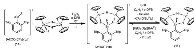
Scheme 13 Synthesis of the hydride bridged trinuclear \text{SnZr}_2 -cation and deprotonation to give 11 ( \text{L} = \text{C}_6\text{H}_6 ).
