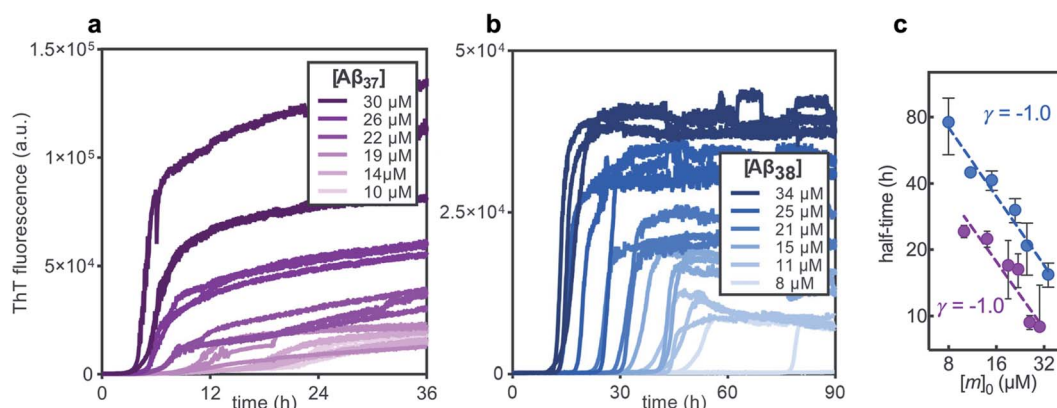
Fig. 3 The aggregation kinetics of pure solutions of (a) A\beta_{37} and (b) A\beta_{38} in 20 mM sodium phosphate buffer, pH 7.4, with 200 \mu M EDTA, 0.02% NaN_3 , and 20 \mu M ThT. Three technical replicates are shown for each concentration. (c) Double-logarithmic plot of the aggregation half-time versus initial monomer concentration, [m]_0 , for A\beta_{37} (purple) and A\beta_{38} (blue), where the half-time is the time at which the fluorescence signal is half of its final plateau value. Each dashed line shows a fitted power function with scaling exponent, \gamma . Points show the mean of the three technical replicates, with error bars showing the standard deviation.
