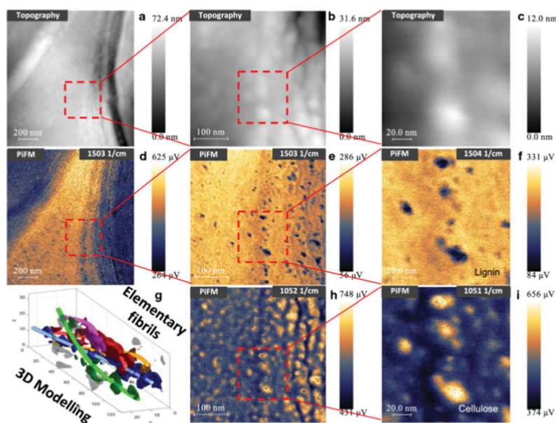
Fig. 10 Topography (a–c) and PiFM images (d–i) of an ultrathin Norway spruce cross-section at ca. 1503 (d–f) and 1052 (h and i) \text{cm}^{-1} at three different magnifications (dimensions shown by the scalebars). A TEM tomography image of a helical cellulose elementary fibrils (EF) bundle with its dimensions (nm) is also shown (g) (Reza et al. 57 ). The vertical cellulose-rich patterns in the PiFM images at ca. 1050\text{ cm}^{-1} may represent tangentially organized EF bundles that are typical of the S_1 layer of Norway spruce tracheids. Reproduced from Kesari et al. 56
